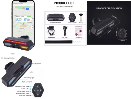
Turning Signal Device with GPS Tracker
